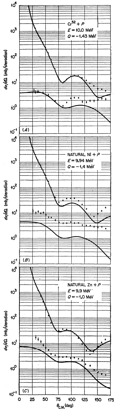
FIG. 7. Experimental and theoretical results at 10 MeV. Model parameters were fixed from Table I and Eqs. (45) and (46). See text for interpretation of the results.
